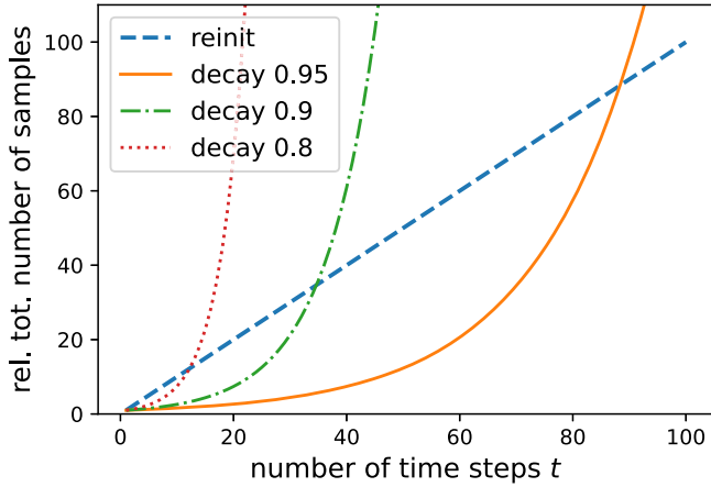
Fig. 12. Comparison of the total number of shots over time for reinitialization methods (dashed line) and our method for different decay factors.
