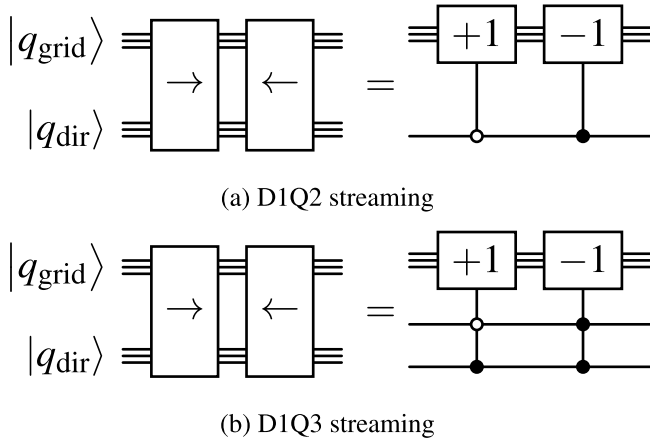
Fig. 7. Arrangement of the controls on the direction qubits for the streaming operations of the D1Q2 scheme (7)(a) and D1Q3 scheme (7)(b).
