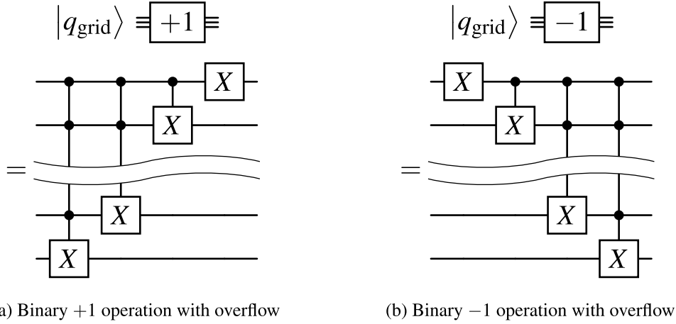
Fig. 6. Binary +1 and -1 operations with overflow as the basis of the right, left, up and down operations in the QLBM circuit in Fig. 2.
